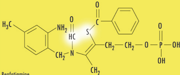
Benfotiamine
